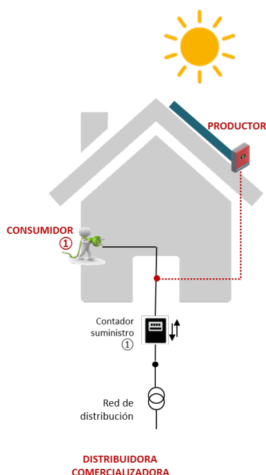
Figura 18: Autoconsumo individual
